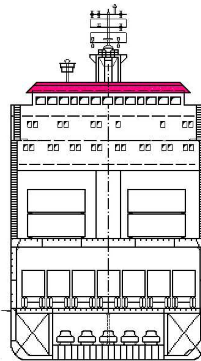
TRANSVERSE SECTION
